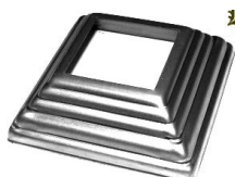
арт. 13.350.01 (100x100x1,2x50)
